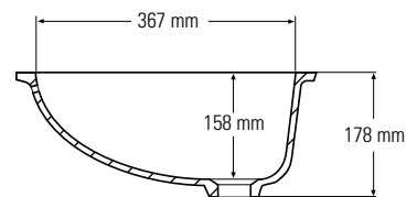
Side cross-section
