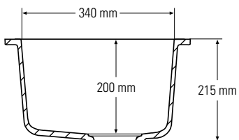
Side cross-section
