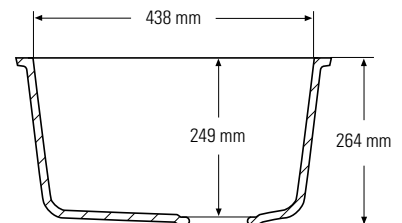
Side cross-section
